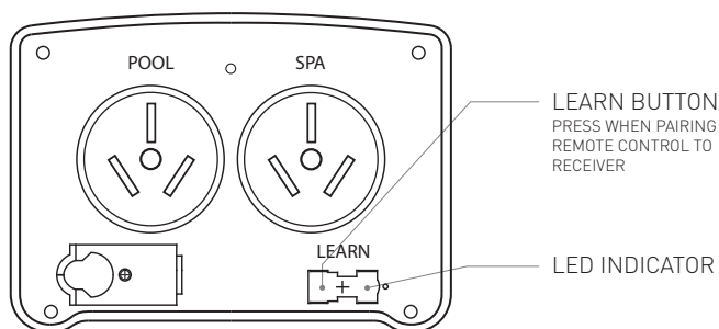
RECEIVER BASE
